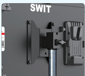
10×10 VESA to Light Stand Adaptor
