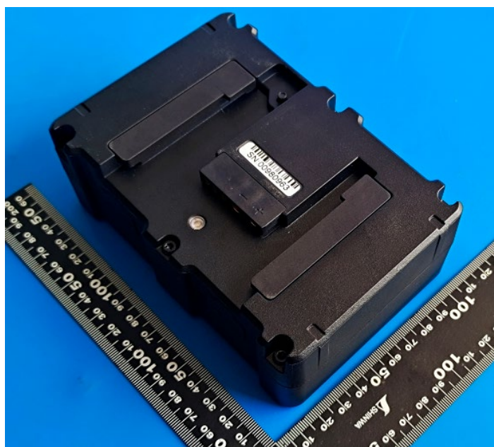
Fig. 2 – Back view of Power Bank 表2-电池反面视图
