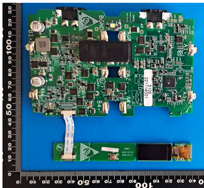
Fig. 6 – Back view of PCM
