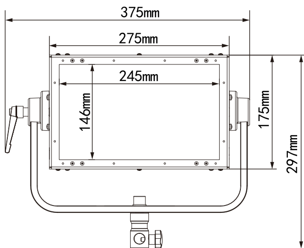
Fig.1 CL-M100C Front View
