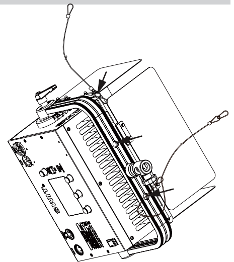
Fig.5 Installation diagram of safety rope
