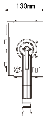
Fig.2 CL-M100C Side View
